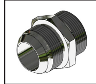
SAE Male to JIC Male Adapter DM80164 Page F7
